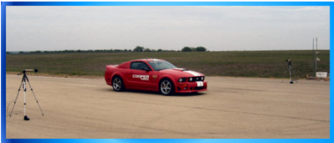
Pass-by-noise testing using GPS technology at Cooper Tire, USA
