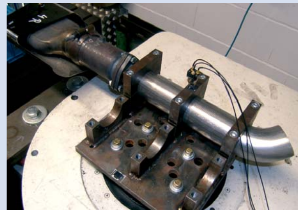
Manifold testing at ArvinMeritor Emissions Technologies GmbH in Augsburg/Germany
