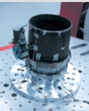
Valve testing at Nord-Micro AG & Co. OHG, Frankfurt
